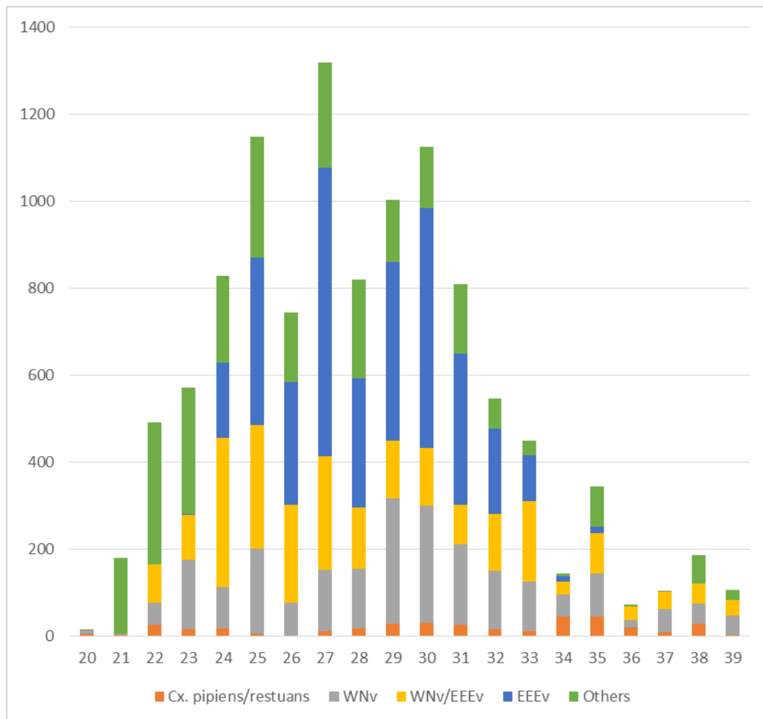
Figure 1. Total identified vector populations from all traps by week. Stacked bar graph displays the total number of mosquitoes identified per week. Y-axis - number of mosquitoes, X-axis - epidemiological week number.
